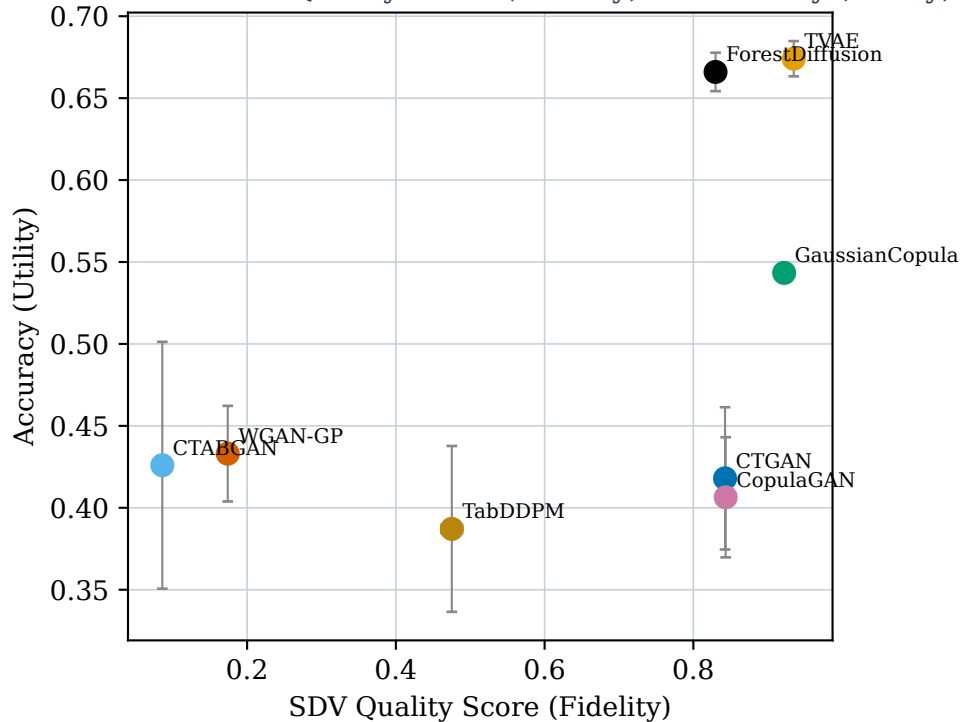
Forest Cover: SDV Quality Score (Fidelity) vs Accuracy (Utility)
